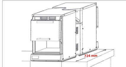
Two units fit back-to-back on a 724 mm (28 1/2") shelf in a 346 mm (13 5/8") space
